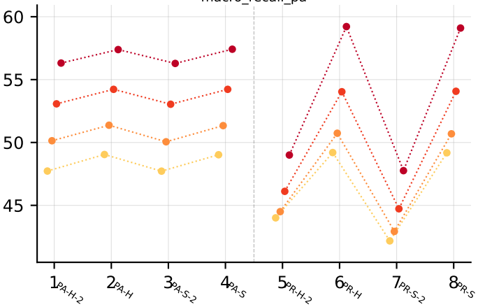
macro_recall_pa
