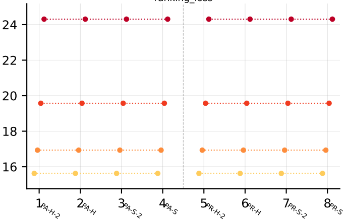
ranking_loss
