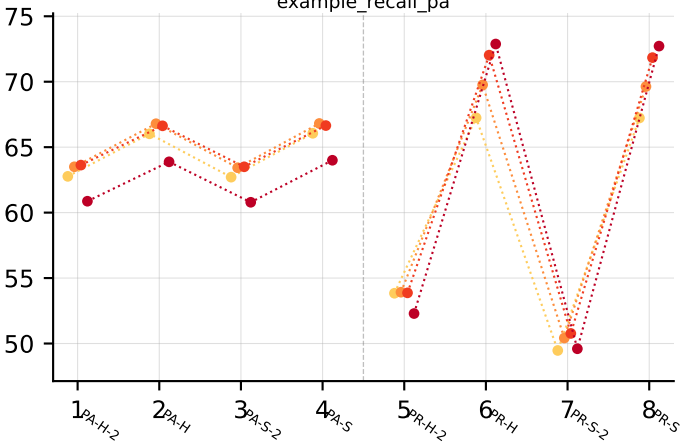
example_recall_pa
