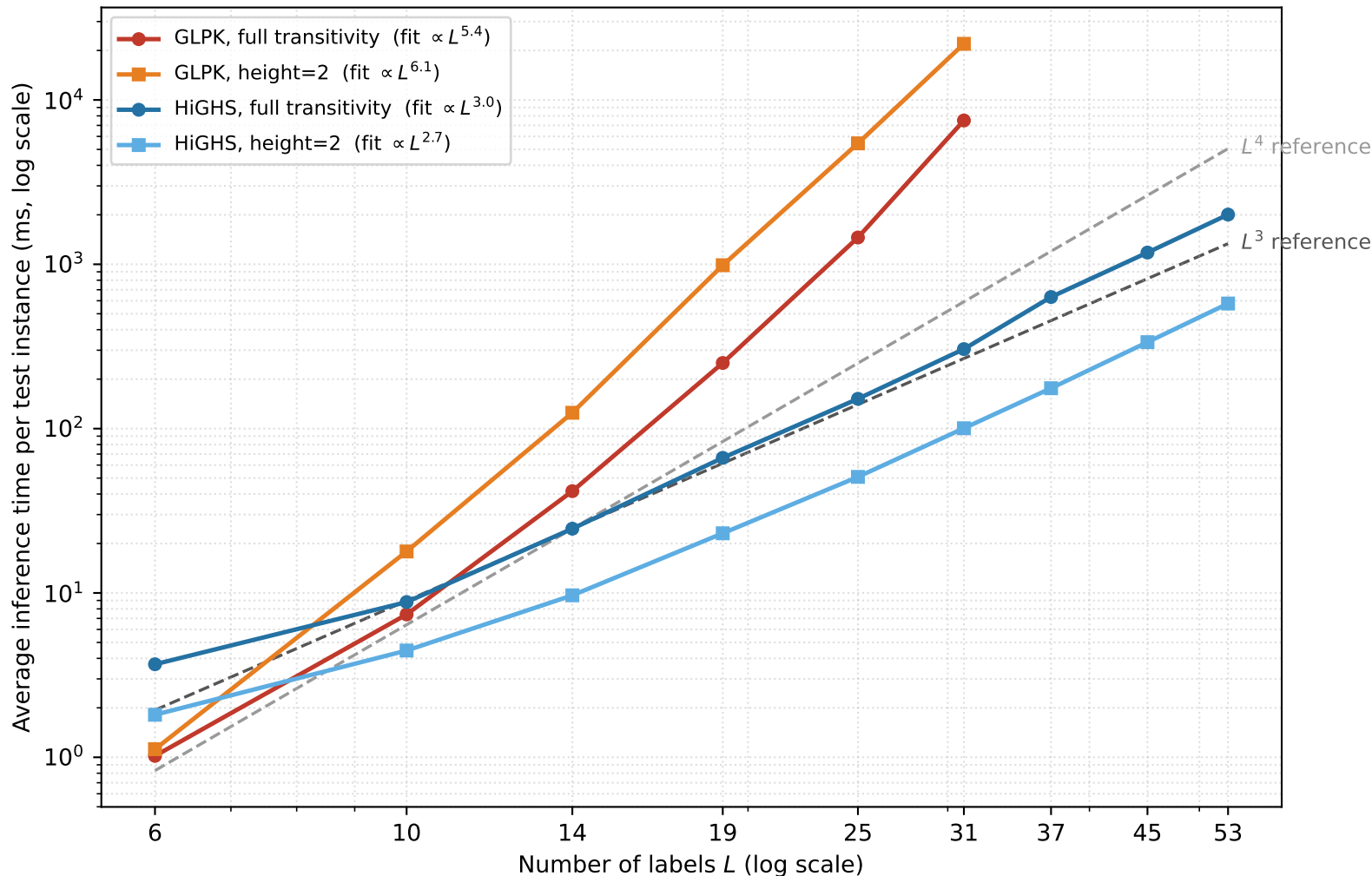
Empirical power-law scaling of the per-instance ILP (real enron RF pairwise probabilities, mean over 300 test instances)
