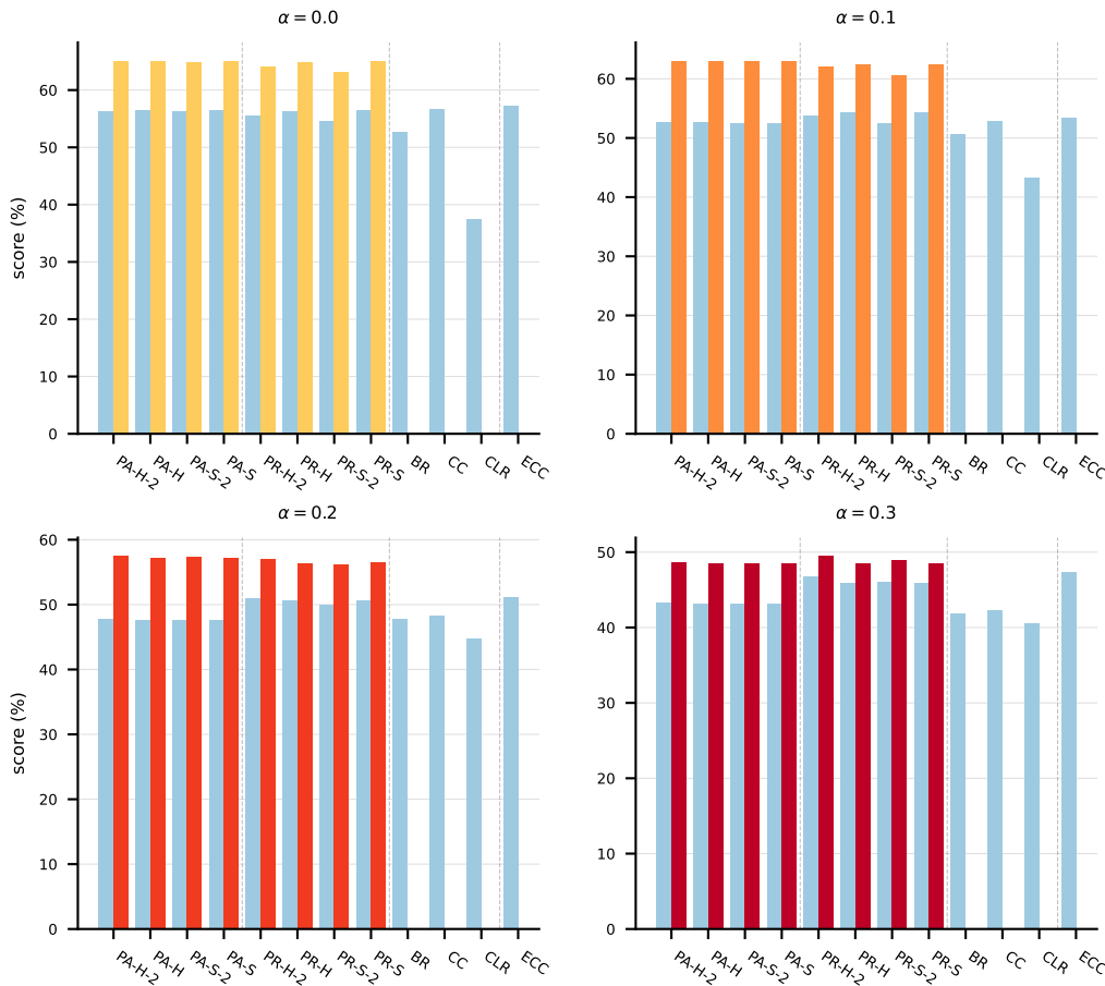
(a) f_1 paired bars
