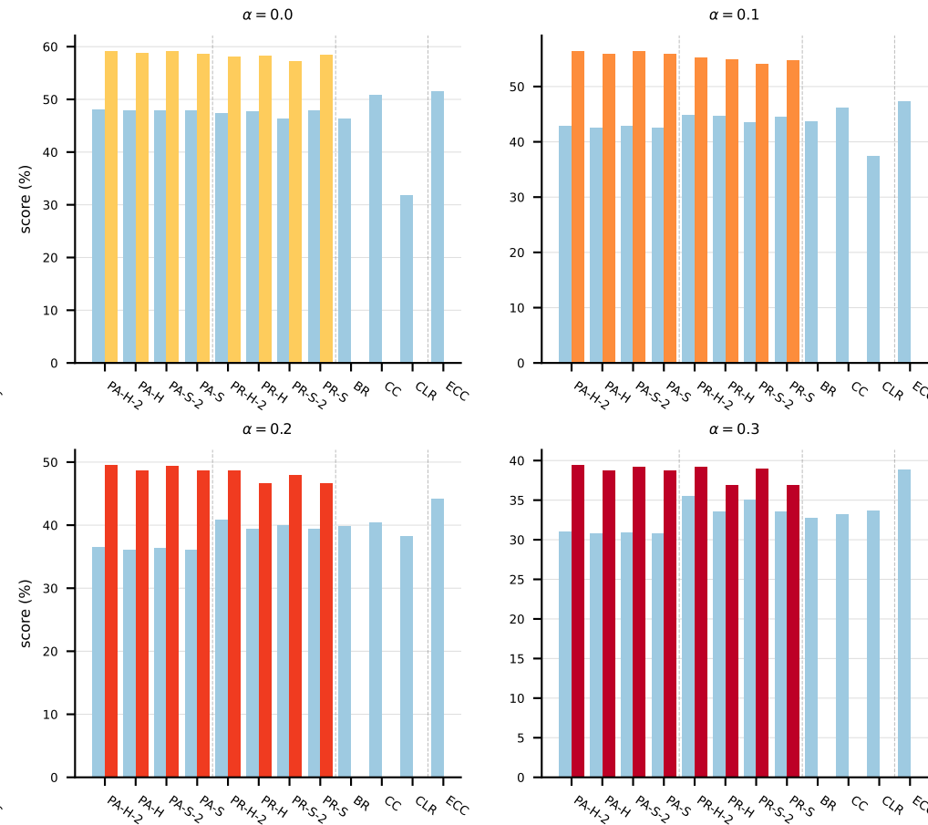
LGBM averaged across all datasets: abstention vs. standard MLC --- detailed by \alpha
