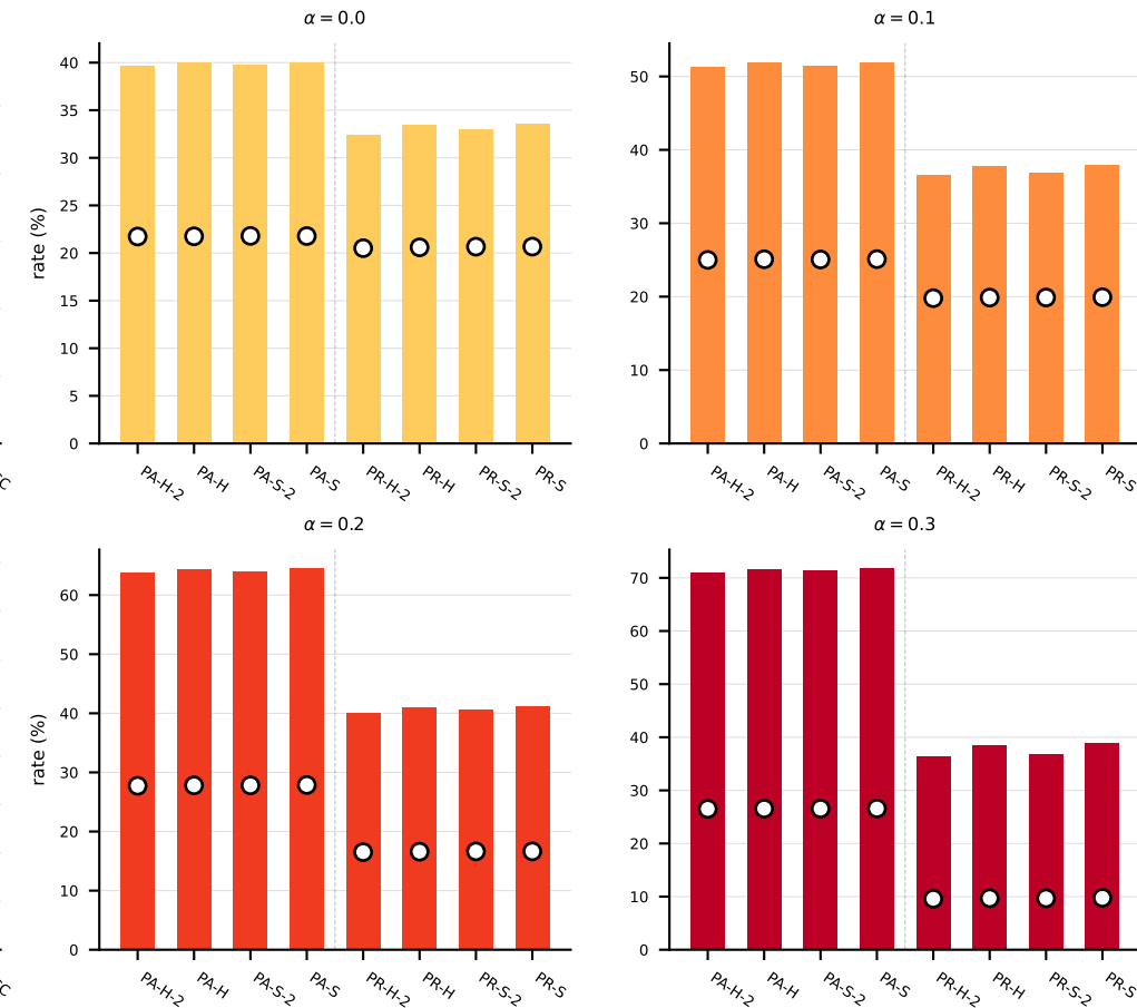
(c) Abstention rates (bar=abs, dot=aabs)
