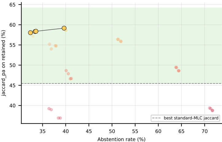
LGBM aggregate (jaccard_pa) -- Pareto frontier + win-region
