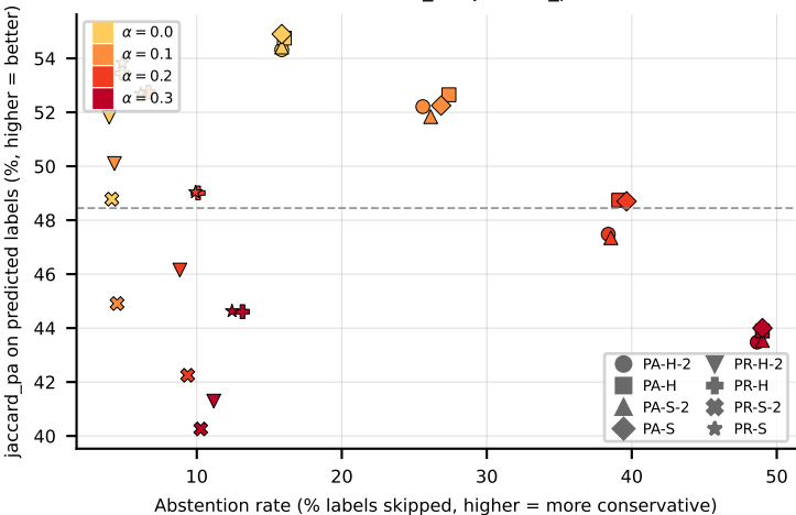
LGBM on CHD_49 (jaccard_pa)
