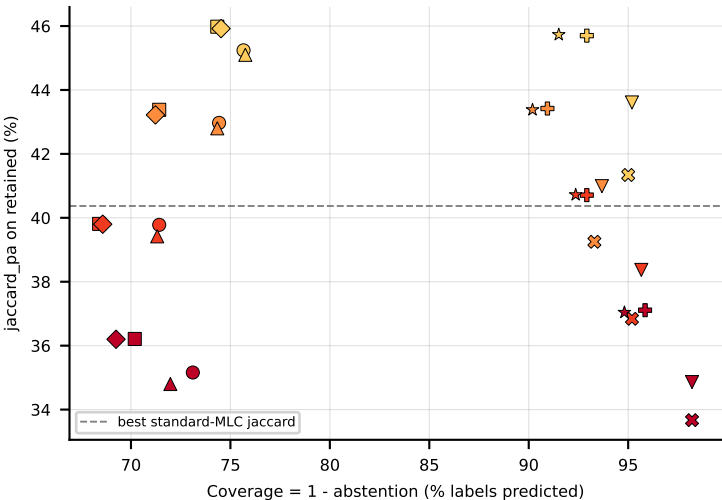
LGBM on Water-quality (jaccard_pa) -- robustness: upper-right = robust
