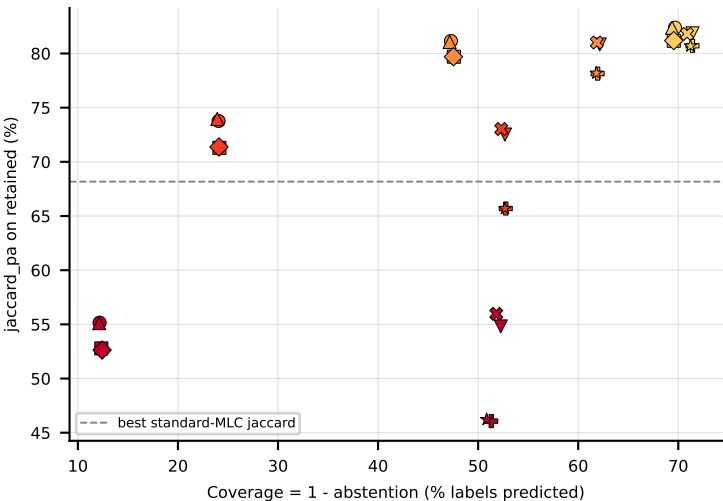
LGBM on scene (jaccard_pa) -- robustness: upper-right = robust
