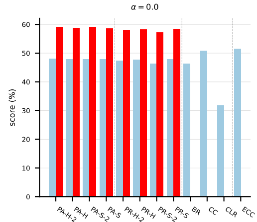
(b) Jaccard paired bars
