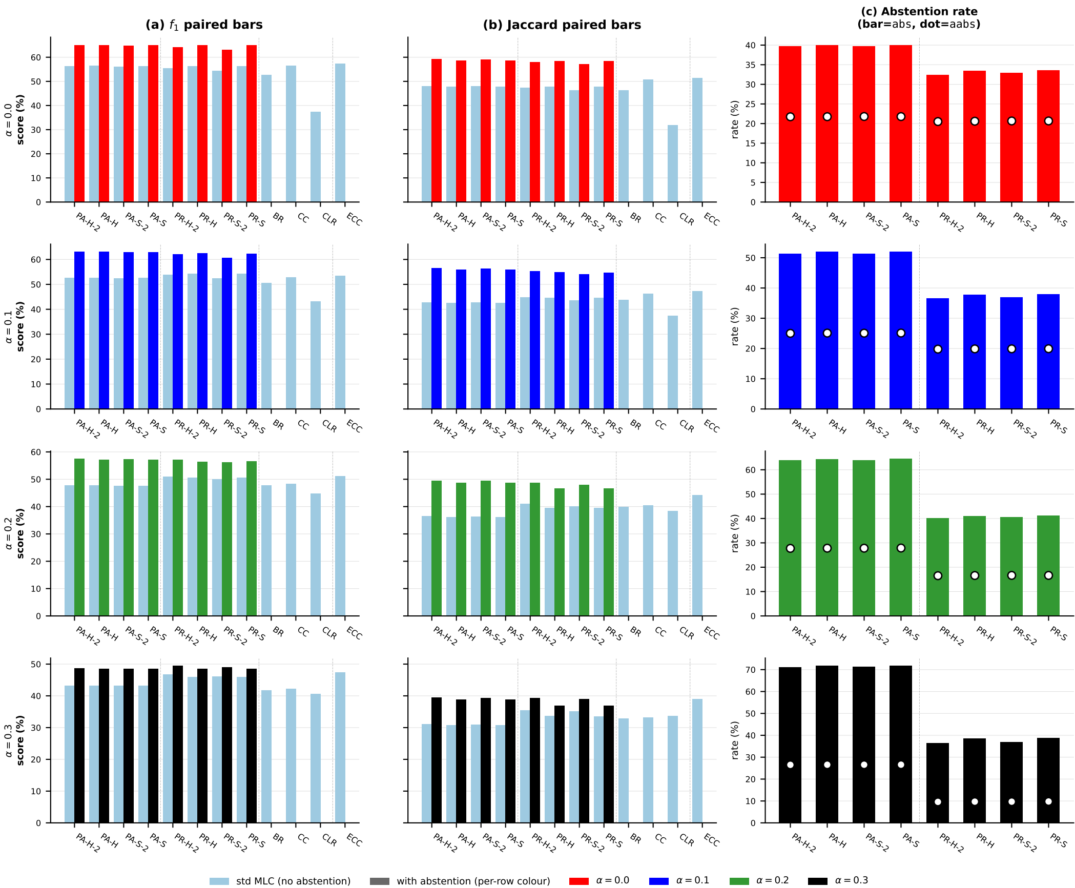
LGBM averaged across all datasets: abstention vs.\ standard MLC --- 4x3 grid
