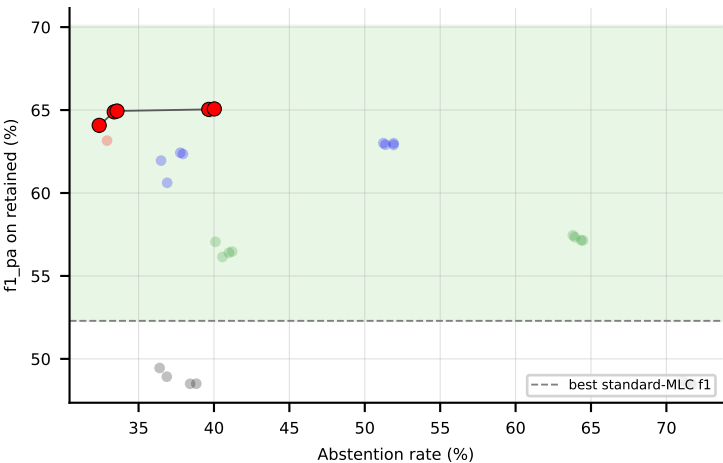
LGBM aggregate (f1_pa) -- Pareto frontier + win-region
