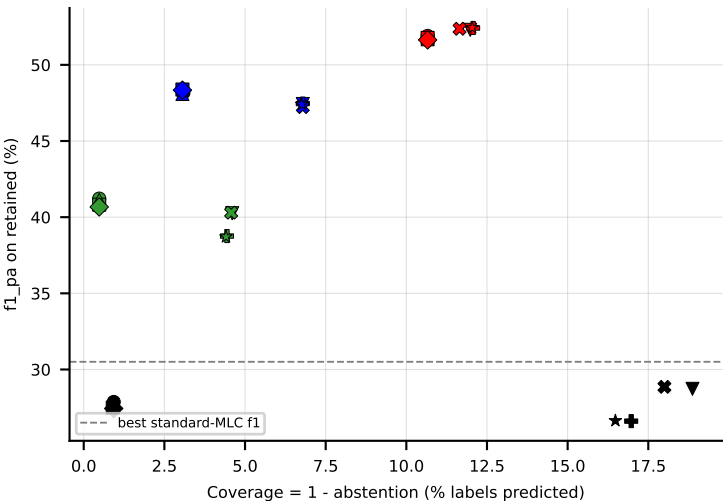
LGBM on HumanPseAAC (f1_pa) -- robustness: upper-right = robust
