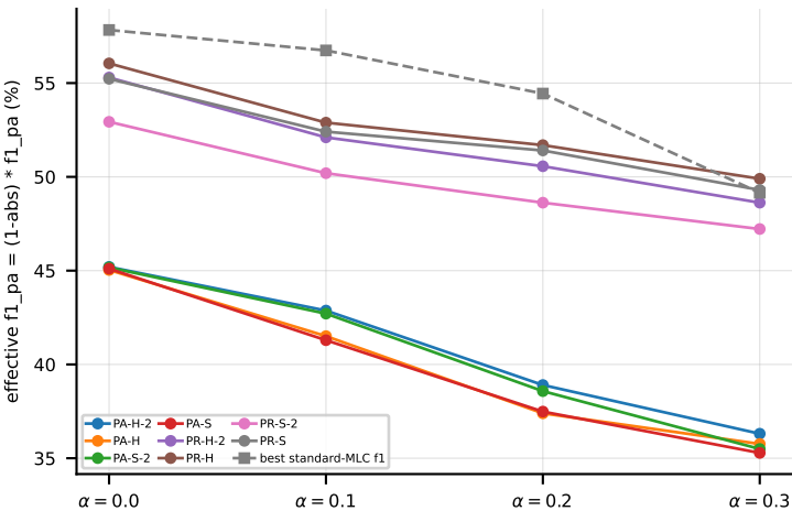
LGBM on Water-quality (f1_pa) -- penalised quality (abstention costs labels)
