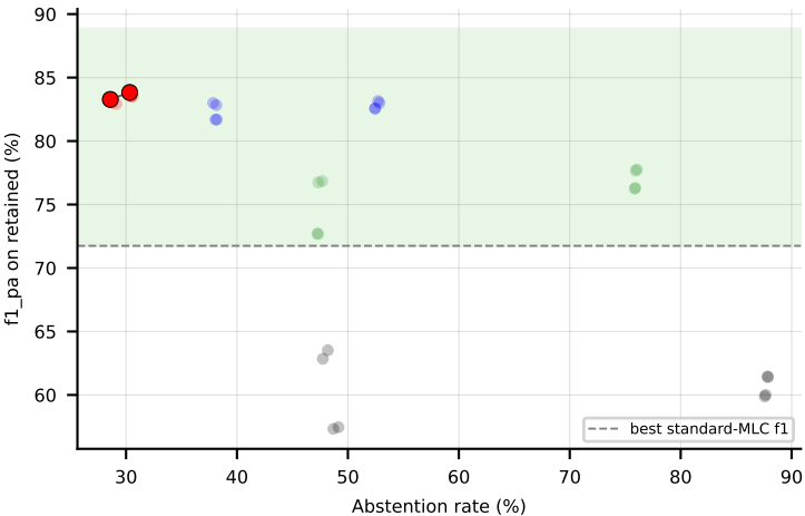
LGBM on scene (f1_pa) -- Pareto frontier + win-region
