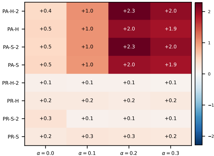
LGBM on Yeast (jaccard_pa) -- gain (jaccard_pa - jaccard, percentage points)
