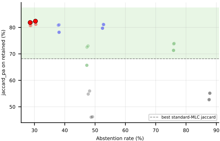
LGBM on scene (jaccard_pa) -- Pareto frontier + win-region
