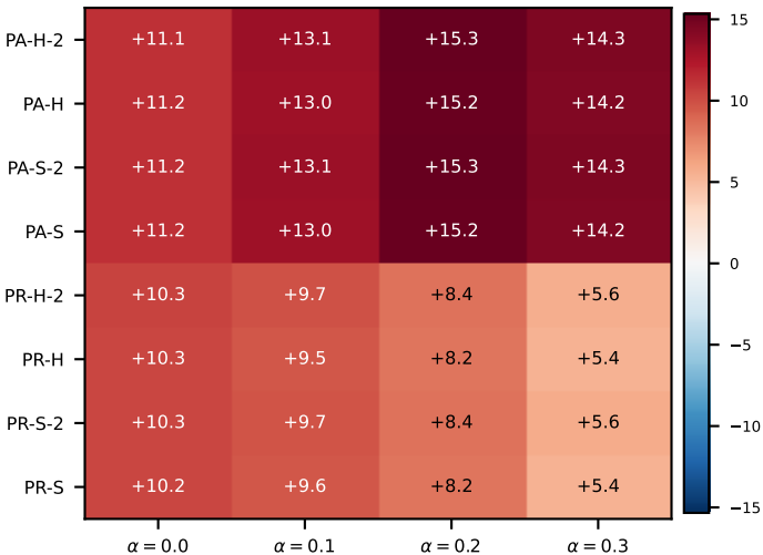
RF aggregate (f1_pa) -- gain (f1_pa - f1, percentage points)
