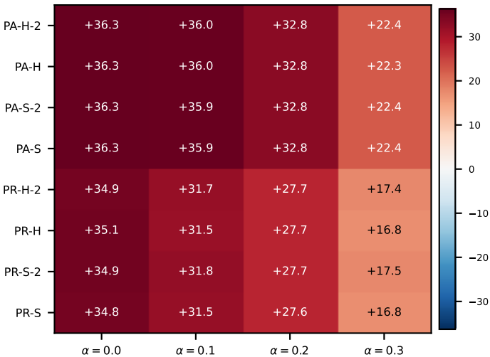
RF on HumanPseAAC (f1_pa) -- gain (f1_pa - f1, percentage points)
