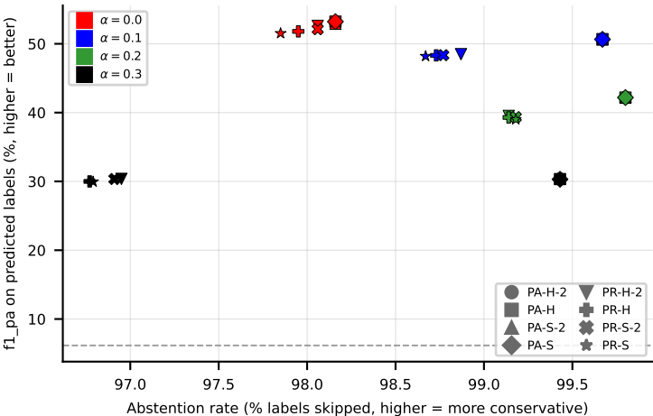
RF on PlantPseAAC (f1_pa)
