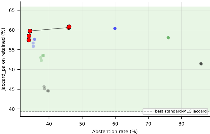
RF aggregate (jaccard_pa) -- Pareto frontier + win-region
