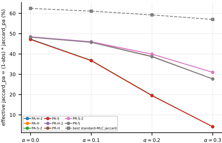
RF on scene (jaccard_pa) -- penalised quality (abstention costs labels)
