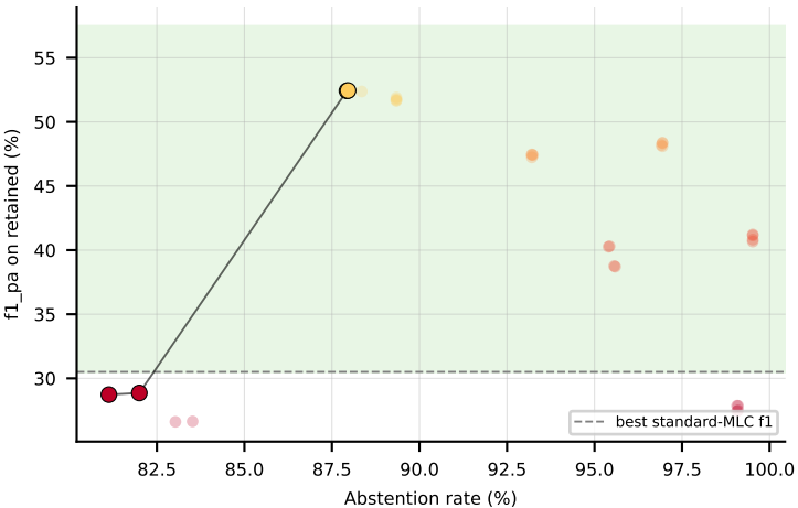
LGBM on HumanPseAAC (f1_pa) -- Pareto frontier + win-region
