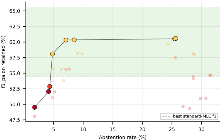
LGBM on Water-quality (f1_pa) -- Pareto frontier + win-region
