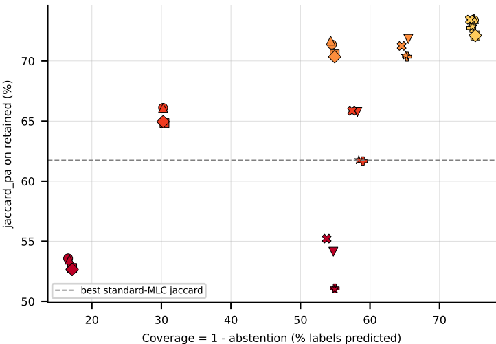
LGBM on GpositivePseAAC (jaccard_pa) -- robustness: upper-right = robust
