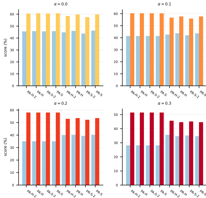
(b) RF averaged across all datasets, abstention vs standard MLC --- detailed by \alpha
