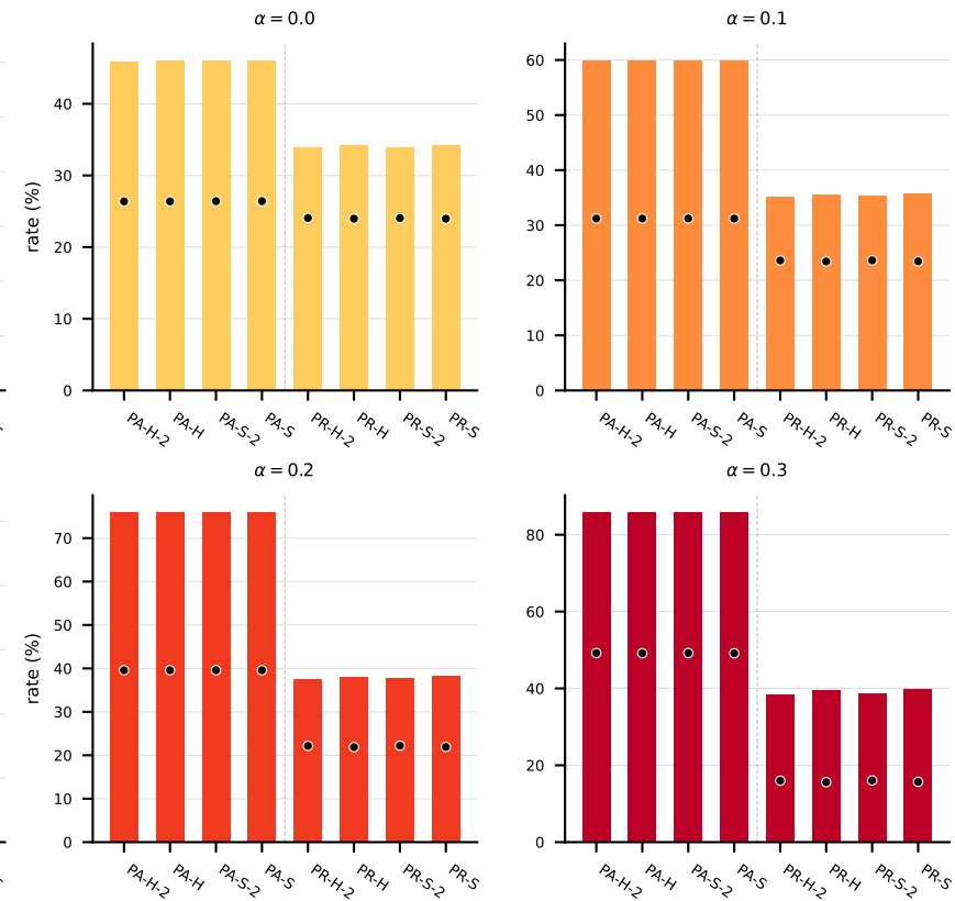
(c) Abstention rates (bar=\texttt{abs}, dot=\texttt{aabs})
