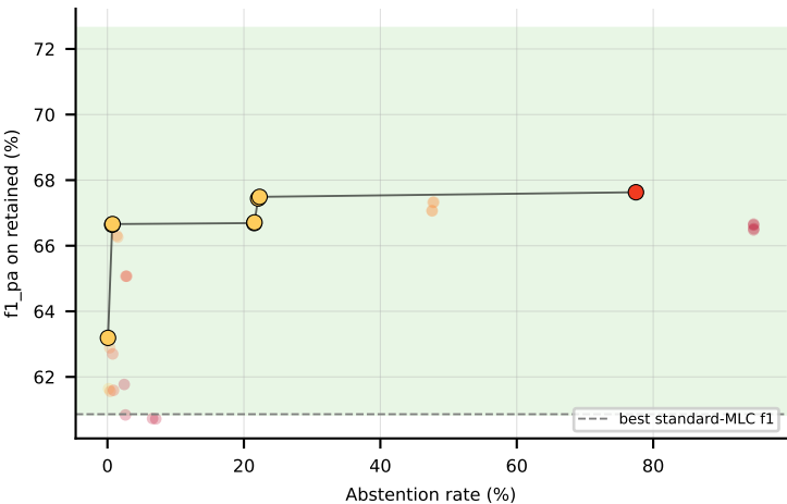
RF on Yeast (f1_pa) -- Pareto frontier + win-region
