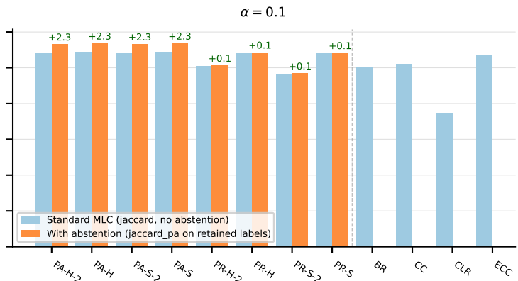
RF on CHD_49 (jaccard_pa)
