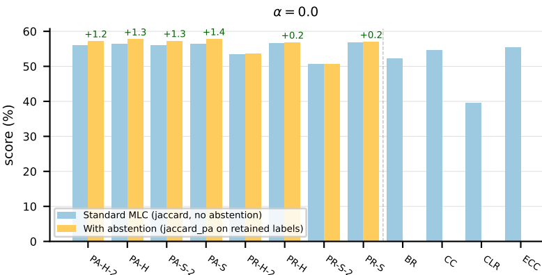
RF on CHD_49 (jaccard_pa)
