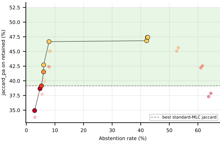
RF on Water-quality (jaccard_pa) -- Pareto frontier + win-region
