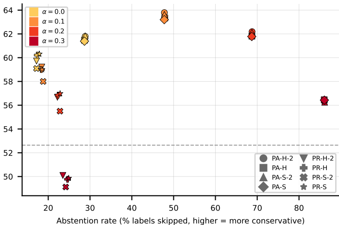
RF on emotions (jaccard_pa)
