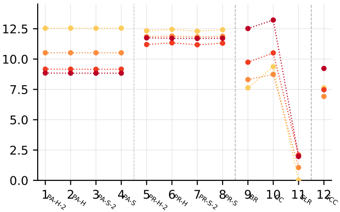
example_precision
