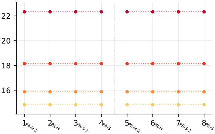
ranking_loss
