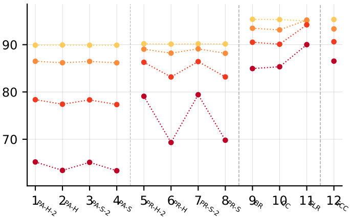
hamming_accuracy
