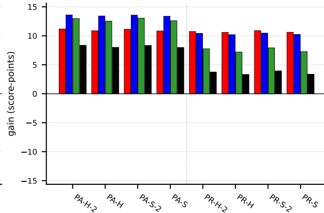
(b) gain on Jaccard: (with-abstention) – (std MLC)
