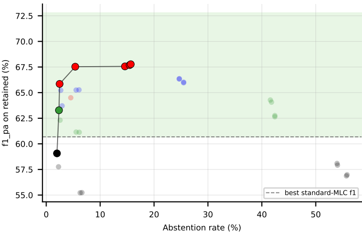
LGBM on Yeast (f1_pa) -- Pareto frontier + win-region
