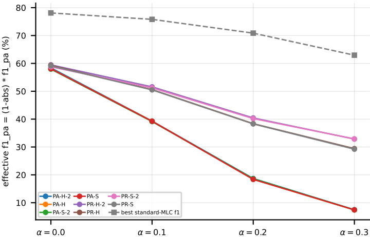
LGBM on scene (f1_pa) -- penalised quality (abstention costs labels)
