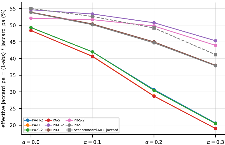
LGBM on Yeast (jaccard_pa) -- penalised quality (abstention costs labels)
