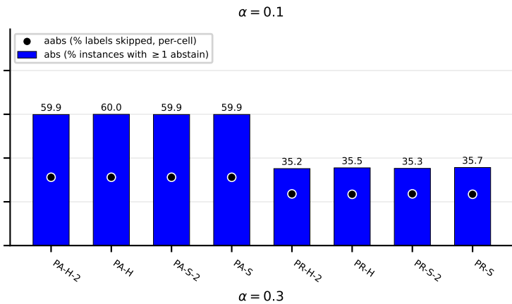
RF aggregate: abstention rates
