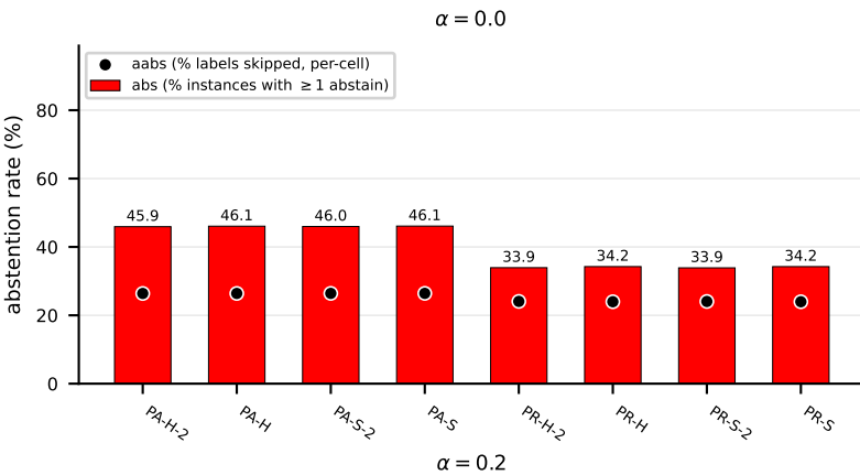
RF aggregate: abstention rates
