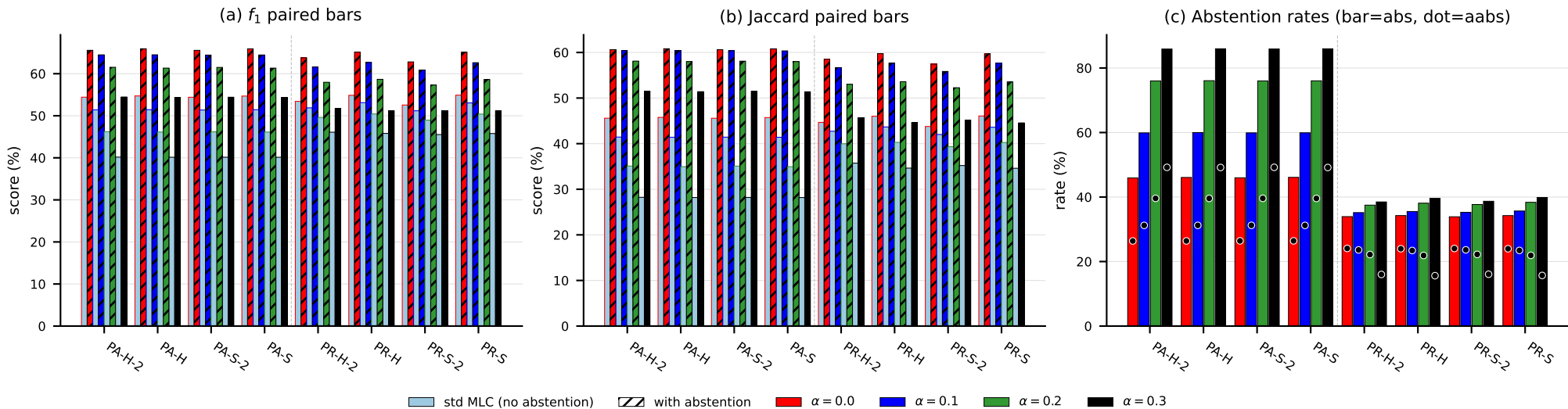
RF averaged across all datasets: abstention summary
