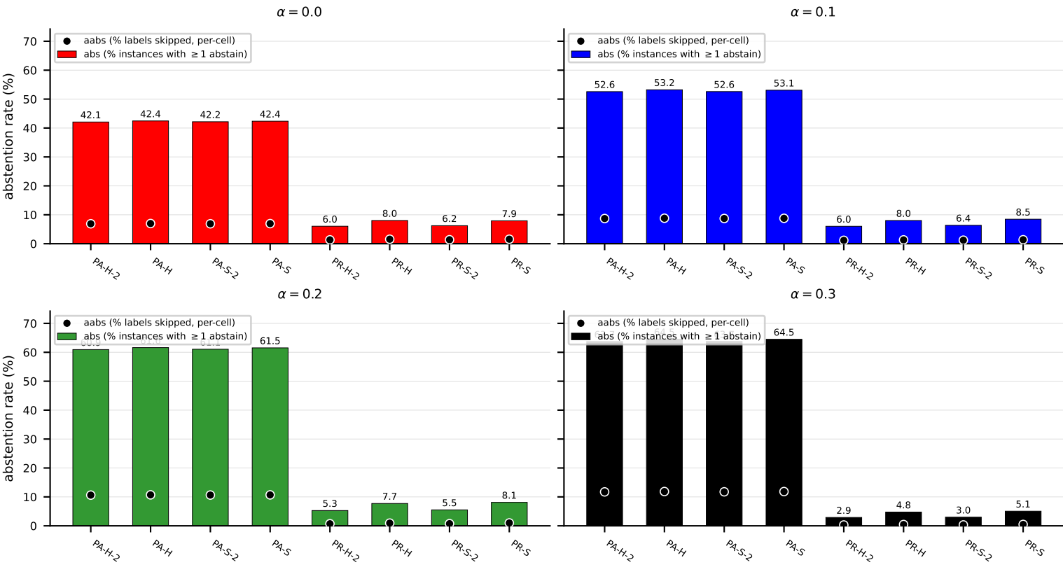
RF on Water-quality: abstention rates
