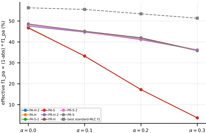
RF on GpositivePseAAC (f1_pa) -- penalised quality (abstention costs labels)
