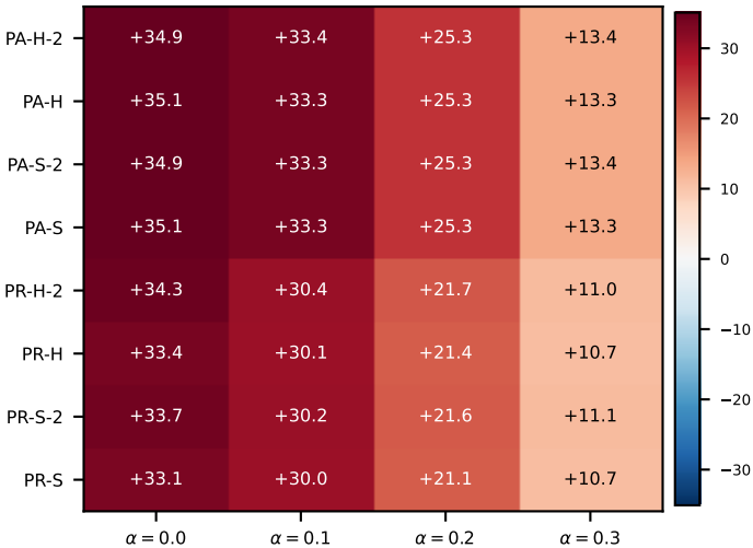
RF on PlantPseAAC (f1_pa) -- gain (f1_pa - f1, percentage points)
