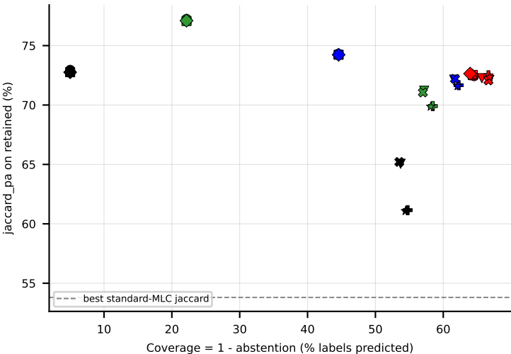
RF on GpositivePseAAC (jaccard_pa) -- robustness: upper-right = robust
