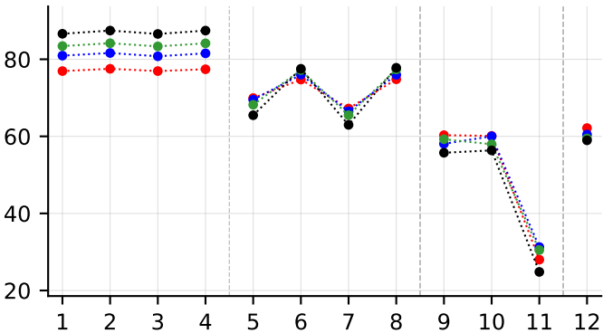
macro_recall
