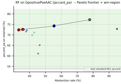
Figure 51: RF (jaccard pa ) on GpositivePseAAC: Pareto frontier of (abstention, retained quality) with the win-region shaded green (left); per-method per-noise gain (jaccard pa − f_1 ) heatmap (right).
