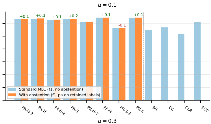
LGBM on CHD_49 (f1_pa)
