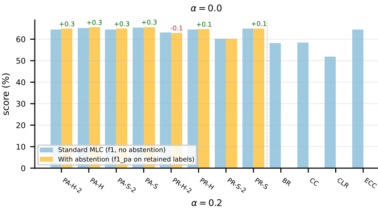
LGBM on CHD_49 (f1_pa)
