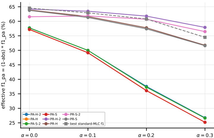
LGBM on Yeast (f1_pa) -- penalised quality (abstention costs labels)
