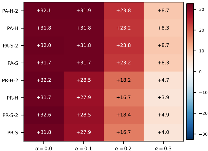
LGBM on HumanPseAAC (jaccard_pa) -- gain (jaccard_pa - jaccard, percentage points)
