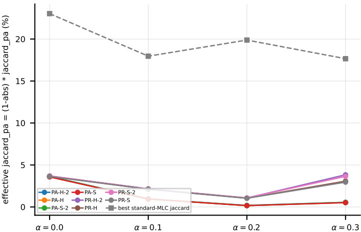
LGBM on PlantPseAAC (jaccard_pa) -- penalised quality (abstention costs labels)
