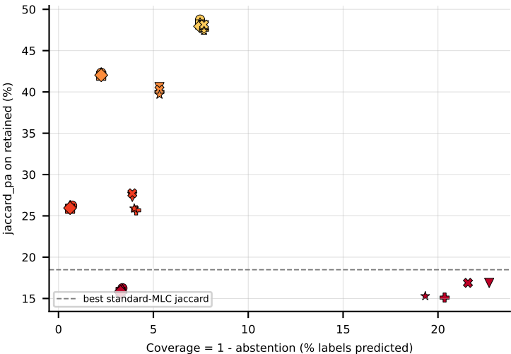
LGBM on PlantPseAAC (jaccard_pa) -- robustness: upper-right = robust
